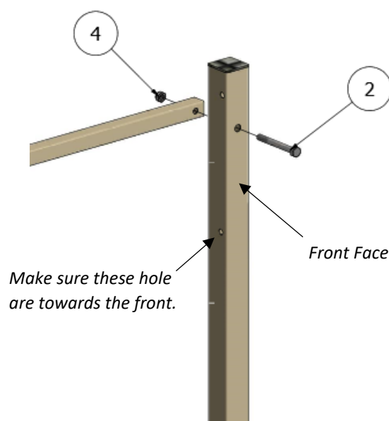
Figure 2 – Bolt Back Bar onto Legs
